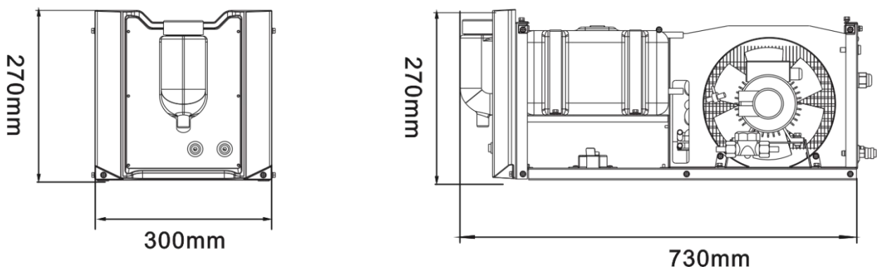
Figure 1-1 Dimension Drawing of Water Cooler
