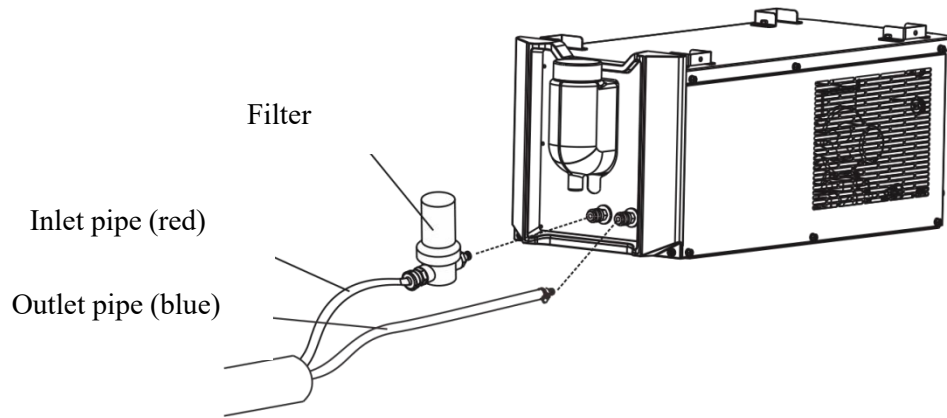
Figure 2-3 Pipe connection diagram of water cooler
