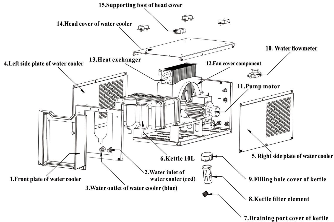
Figure 1 Structure Diagram
