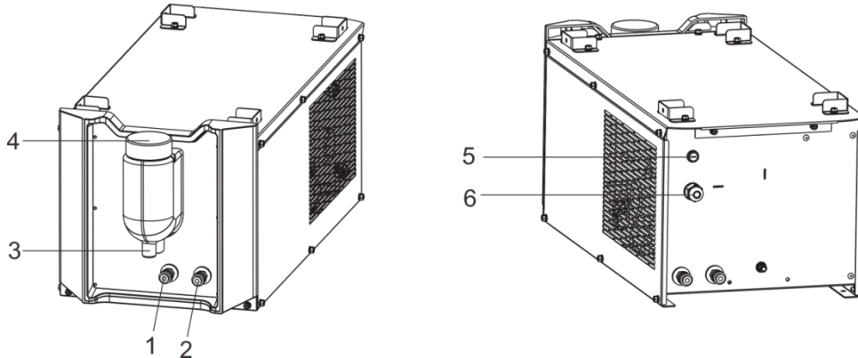
Figure 3-1 Water cooler part drawing
